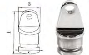
AISI316 STAINLESS STEEL TOP CAP 316不锈钢球形滑帽
