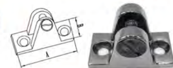
AISI316 STAINLESS STEEL DECK HINGE 90° 316不锈钢重型山型座
