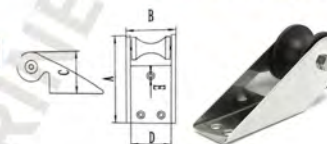
AISI316 STAINLESS STEEL BOW ROLLER 316不锈钢黑色单轮锚支架
