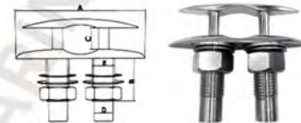
AISI316 STAINLESS STEEL HEAVY POP UP CLEAT 316不锈钢隐形索栓
