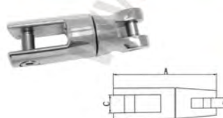
AISI316 STAINLESS STEEL ANCHOR DOUBLE CONNECTOR 316不锈钢两段锚链连接器
