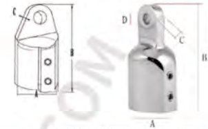
AISI316 STAINLESS STEEL TOP CAP 316不锈钢单弯滑帽
