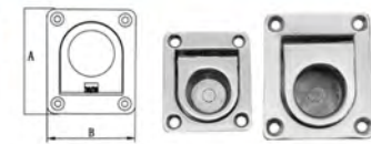
AISI316 STAINLESS STEEL HEAVY SQUARE FLUSH LIFT RING WITH SPRING 316不锈钢重型地板拉环
