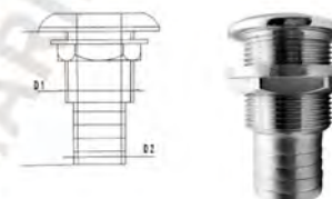
AISI316 STAINLESS STEEL THRU-HULL WITH HOSE 316不锈钢加长半丝出水口
