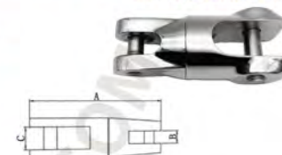
AISI316 STAINLESS STEEL HEAVY ANCHOR DOUBLE CONNECTOR 316不锈钢重型两段锚链连接器
