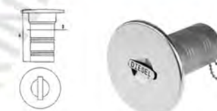
AISI316 STAINLESS STEEL DECK FILLER 316不锈钢弯盖油箱体
