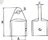
AISI316 STAINLESS STEEL TOP CAP 316不锈钢单顶丝滑帽
