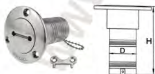
AISI316 STAINLESS STEEL DECK FILLER (WITH KEY) 316不锈钢带钥匙油箱体
