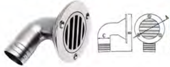
AISI316 STAINLESS STEEL COCKPIT 316不锈钢可拆卸弯地漏
