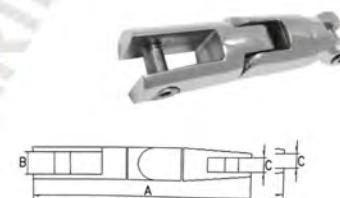
AISI316 STAINLESS STEEL ANCHOR CONNECTOR 316不锈钢长锚链连接器
