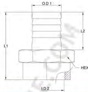
Female & Barbed Fitting-2
