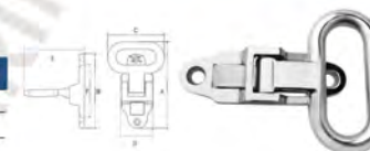
AISI316 STAINLESS STEEL FOLDING STEP 316不锈钢沉孔马蹄蹬/脚踏
