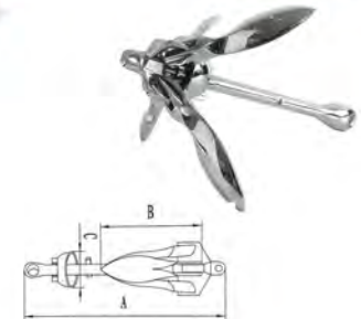
AISI316 STAINLESS STEEL GRAPNEL ANCHOR 316不锈钢伞锚/折叠锚
