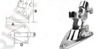
AISI316 STAINLESS STEEL MIRROR POLISHED FLAGPOLE BASE 316不锈钢镜面抛光旗杆座
