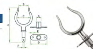
STAINLESS STEEL ROW LOCK 316不锈钢桨叉
