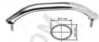
S/S HEAVY DUTY OVAL HANDRAIL S/S重型椭圆形扶手
