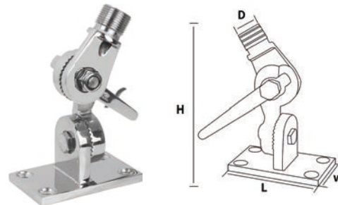
AISI316 STAINLESS STEEL HEAVY ANTENNA BASE 316不锈钢天线座重型
