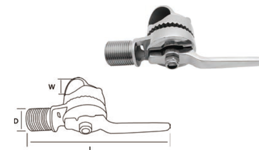
AISI316 STAINLESS STEEL ANTENNA BASE 316不锈钢天线座
