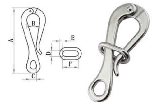
QUICK RELEASE HOOK 释放钩
