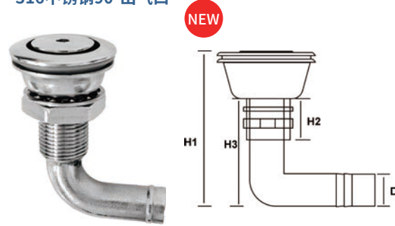
AISI316 STAINLESS STEEL 90° TANK VENT 316不锈钢90°出气口
