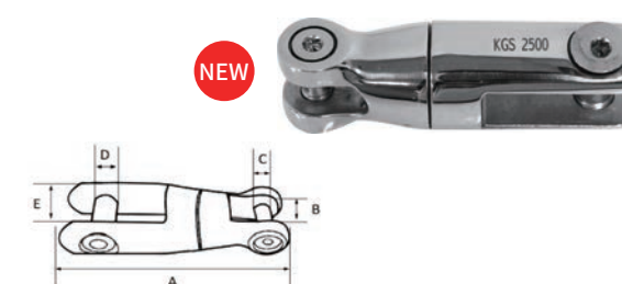
AISI316 STAINLESS STEEL ANCHOR TRIPLE CONNECTOR 316不锈钢三段锚链接器
