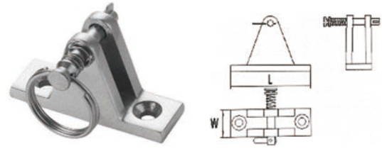
316 STAINLESS STEEL CONCAVE BASE DECK HINGE 316不锈钢弧型小山型座
