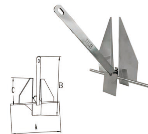
AISI316 STAINLESS STEEL DANFORTH ANCHOR 316不锈钢丹弗斯锚
