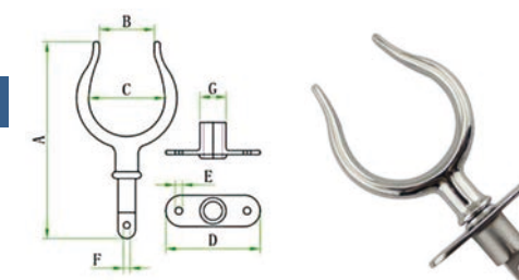
AISI316 STAINLESS STEEL ROW LOCK 316不锈钢桨叉
