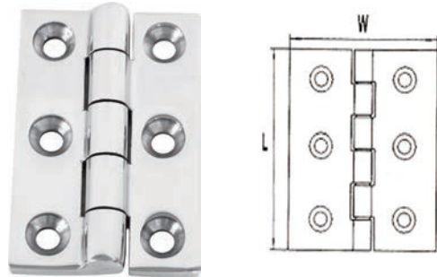
AISI316 STAINLESS STEEL CASTING HINGE 316不锈钢对称合页
