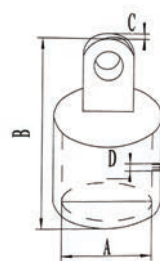
AISI316 STAINLESS STEEL BIMINI TOP CAP 316不锈钢三角双顶丝滑帽
