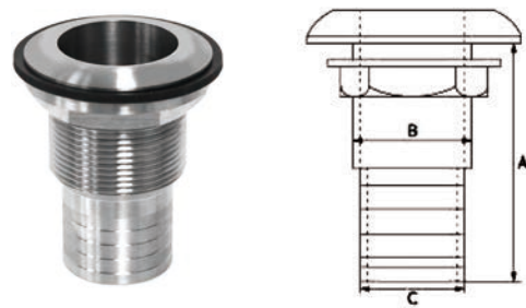
THRU HULL OUTLET WITH CHECK VALVE 带止回阀半丝出水口
