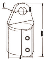
AISI316 STAINLESS STEEL BIMINI TOP CAP 316不锈钢单顶丝滑帽
