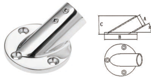
AISI316 STAINLESS STEEL HANDRAIL 30°ROUND BASE 316不锈钢30°圆管座
