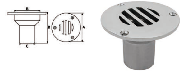
AISI316 STAINLESS STEEL COCKPIT DRAIN 316不锈钢焊接直地漏
