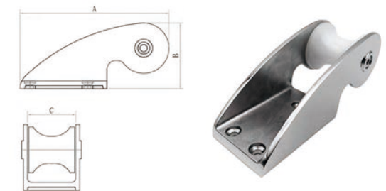
AISI316 STAINLESS STEEL HINGED BOW ROLLER 316不锈钢锚支架
