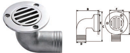
AISI316 STAINLESS STEEL 90° COCKPIT DRAIN 316不锈钢一体弯地漏
