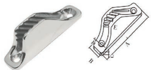
AISI316 STAINLESS STEEL CLEATS INOX FOR ROPES 316不锈钢夹绳器
