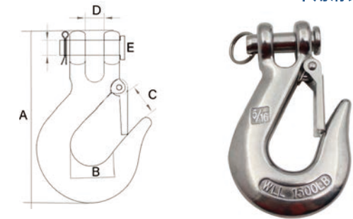
CRANE HOOK WITH LATCH 羊角滑钩
