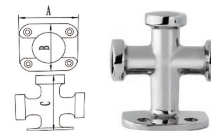
AISI316 STAINLESS STEEL DOUBLE CROSS BOLLARD 316不锈钢双十字缆桩
