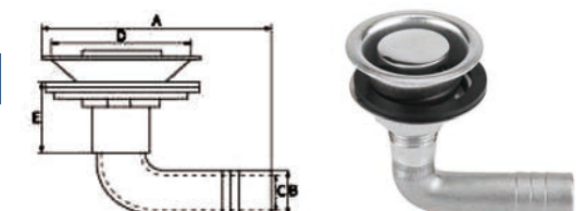
AISI316 STAINLESS STEEL 90° TANK VENT WITH CAP 316不锈钢90°大盖出水口
