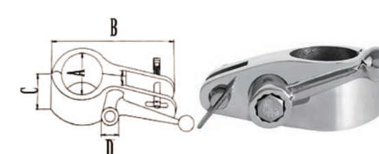
AISI316 STAINLESS STEEL BIMINI TOP SLIDE 316不锈钢球形把手螺栓管夹
