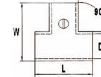
AISI316 STAINLESS STEEL 90°HANDRAIL TEE 316不锈钢90°开口三通
