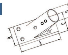
AISI316 STAINLESS STEEL HANDRAIL 30°RECTANGULAR BASE 316不锈钢30°方管座
