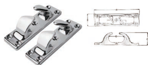
AISI316 STAINLESS STEEL BOW CHOCK 316不锈钢直导缆器
