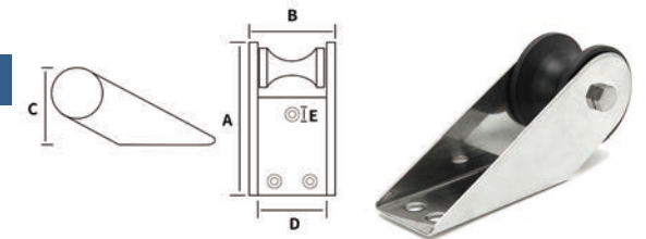
AISI316 STAINLESS STEEL BOW ROLLER 316不锈钢黑色单轮锚支架
