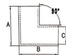
AISI316 STAINLESS STEEL 90°ELBOW 316不锈钢90°弯头
