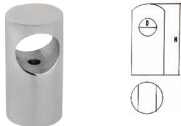
AISI316 STAINLESS STEEL END FITTING FOR HANDRAIL 316不锈钢盲孔支架
