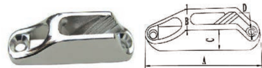
AISI316 STAINLESS STEEL CLEATS INOX FOR ROPES 3/6MM 316不锈钢夹绳器
