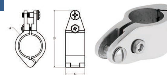
AISI316 STAINLESS STEEL BIMINI TOP SLIDE WITH PIN 316不锈钢销子管夹
