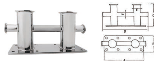
AISI316 STAINLESS STEEL DOUBLE CROSS BOLLARD 316不锈钢双十字缆桩
