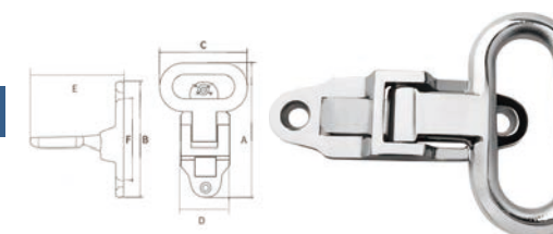
AISI316 STAINLESS STEEL MARINE FOLDING STEP 316不锈钢沉孔马蹄蹬/脚踏
