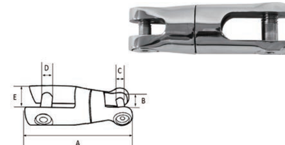
AISI316 STAINLESS STEEL ANCHOR DOUBLE CONNECTOR 316不锈钢两段锚链接器
