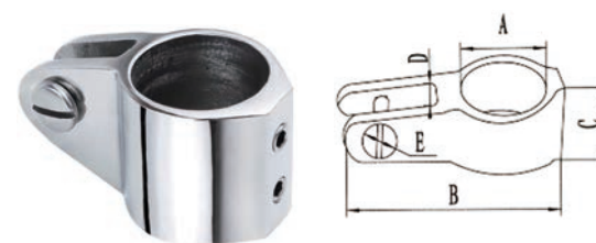
AISI316 STAINLESS STEEL BIMINI TOP SLIDE 316不锈钢带棱角双顶丝滑套
