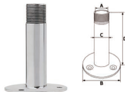
AISI316 STAINLESS STEEL ANTENNA BASE 316不锈钢天线座
