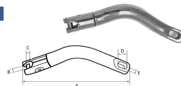
AISI316 STAINLESS STEEL ANCHOR CONNECTOR 316不锈钢长锚链接器
