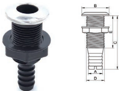
THRU-HULL WITH HOSE 直半丝出水口
