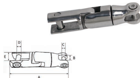
AISI316 STAINLESS STEEL ANCHOR CONNECTOR 316不锈钢长锚链接器
