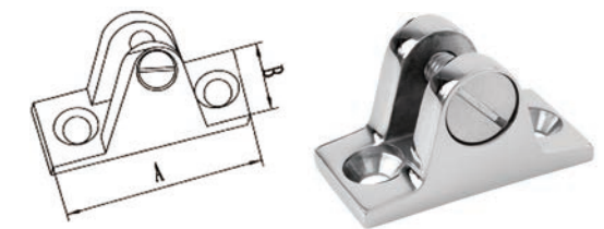
316 STAINLESS STEEL DECK HINGE 90° 316不锈钢弧型大山型座
