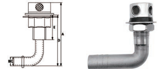
AISI316 STAINLESS STEEL 90° TANK VENT 316不锈钢90°出水口
