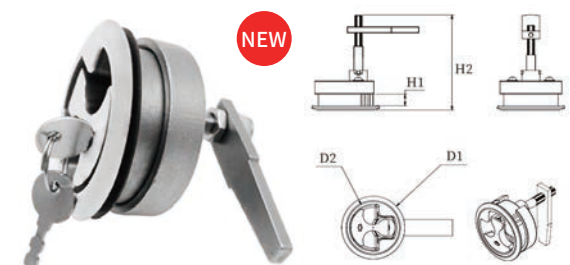
AISI316 STAINLESS STEEL TURNING LOCK WITH KEY(UPGRADED WATEEPROOF) 316不锈钢带钥匙防水地板锁
