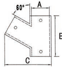
AISI316 STAINLESS STEEL 60°RIGHT HANDRAIL TEE 316不锈钢60°右侧三通
