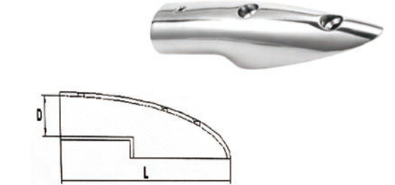
AISI316 STAINLESS STEEL RAIL END 316不锈钢羊蹄支架
