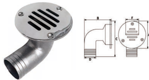
AISI316 STAINLESS STEEL REMOVABLE COCKPIT DRAIN 316不锈钢可拆卸直地漏
