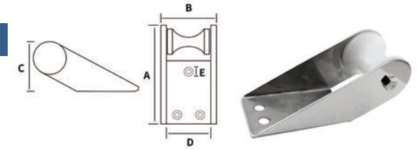
AISI316 STAINLESS STEEL BOW ROLLER 316不锈钢白色单轮锚支架
