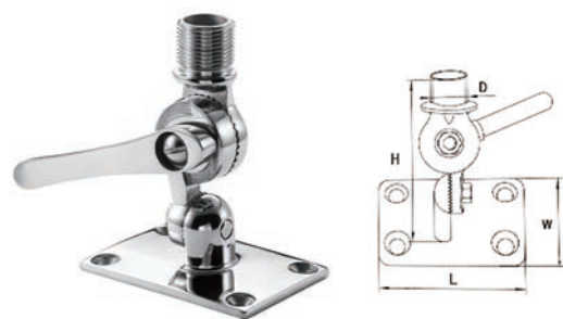
AISI316 STAINLESS STEEL HEAVY ANTENNA BASE 316不锈钢天线座重型
