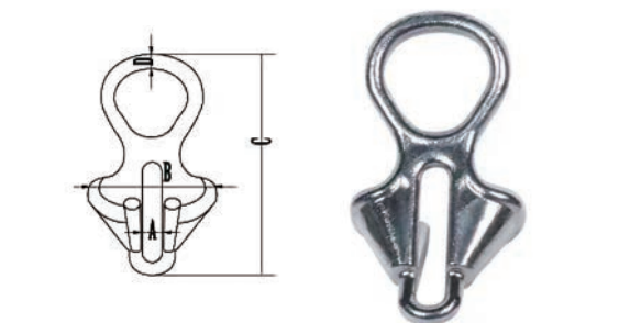
AISI316 STAINLESS STEEL HEAVY ANCHOR CHAIN LOCK 316不锈钢重型止链器
