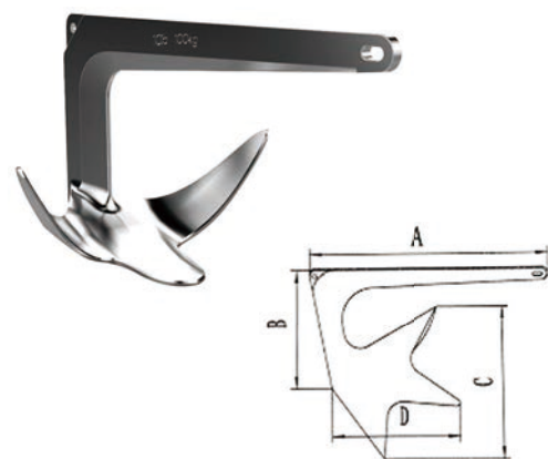
AISI316 STAINLESS STEEL BRUCE ANCHOR 316不锈钢布鲁斯锚
