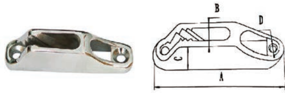
AISI316 STAINLESS STEEL CLEATS INOX FOR ROPES 3/6MM 316不锈钢夹绳器
