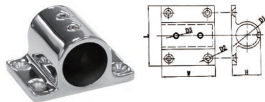
AISI316 STAINLESS STEEL RECTANGLE STANCHION BASE 316不锈钢方底座支架
