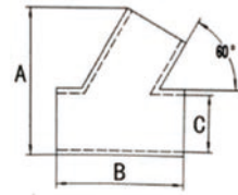
AISI316 STAINLESS STEEL 60°LEFT HANDRAIL TEE 316不锈钢60°左侧三通
