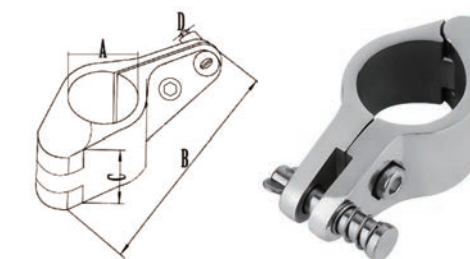
AISI316 STAINLESS STEEL HEAVY BIMINI TOP SLIDE 316不锈钢重型螺栓管夹
