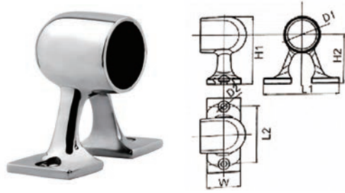
AISI316 STAINLESS STEEL HANDRAIL STANCHION (FORWARD/END 90°) 316不锈钢前/后船支架
