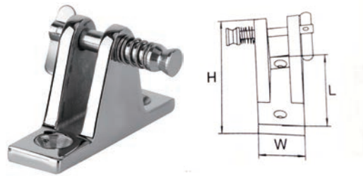
316 STAINLESS STEEL DECK HINGE 90°-REMOVABLE 316不锈钢带环90°销子山型座
