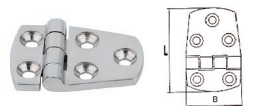
AISI316 STAINLESS STEEL CASTING HINGE 316不锈钢合页
