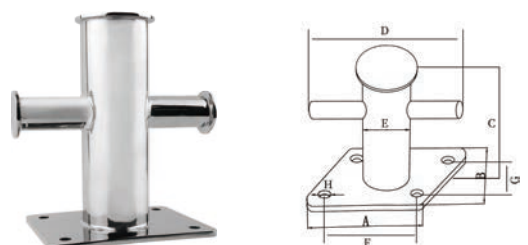
AISI316 STAINLESS STEEL SINGLE CROSS BOLLARD 316不锈钢单十字缆桩
