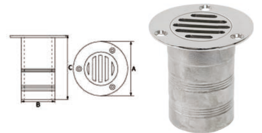
AISI316 STAINLESS STEEL COCKPIT DRAIN SCUPPER WITH BALL 316不锈钢浮球地漏
