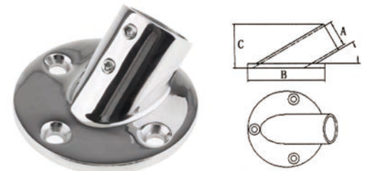
AISI316 STAINLESS STEEL HANDRAIL 45°ROUND BASE 316不锈钢45°圆管座
