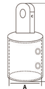
AISI316 STAINLESS STEEL BIMINI TOP CAP 316不锈钢单弯滑帽
