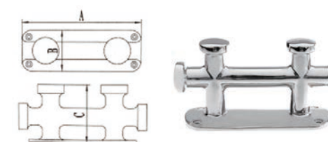
AISI316 STAINLESS STEEL SINGLE BOLLARD 316不锈钢心形缆桩
