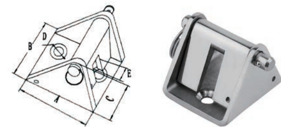
AISI316 STAINLESS STEEL ANCHOR CHAIN STOPPER 316山型止链器
