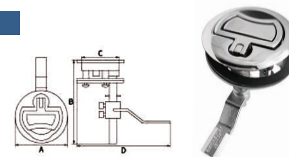
AISI316 STAINLESS STEEL TURNING LOCK 316不锈钢D型弹簧锁
