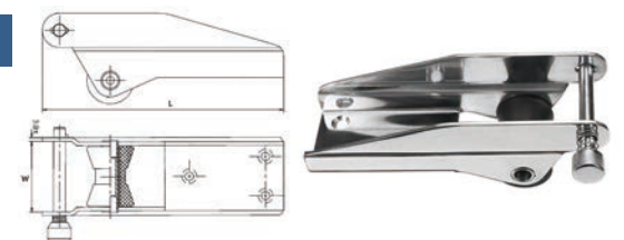
AISI316 STAINLESS STEEL HINGED BOW ROLLER 316不锈钢锚支架
