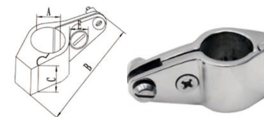
AISI316 STAINLESS STEEL HEAVY BIMINI TOP SLIDE 316不锈钢重型螺栓管夹
