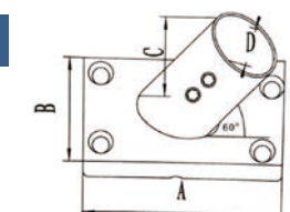
AISI316 STAINLESS STEEL HANDRAIL 60°RECTANGULAR BASE 316不锈钢60°方管座
