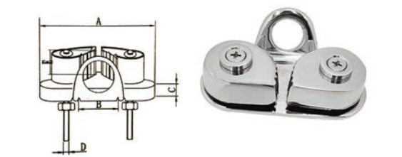
AISI316 STAINLESS STEEL ROPE CLAMP CAM CLEAT 316不锈钢带导向孔快速夹绳器
