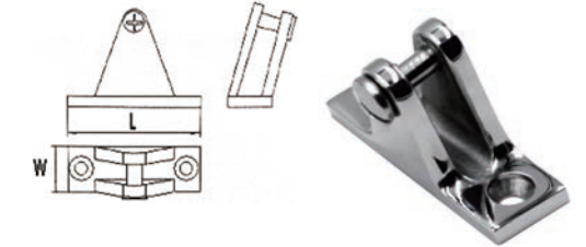
316 STAINLESS STEEL DECK HINGE 60°-REMOVABLE PIN 316不锈钢斜销子山型座
