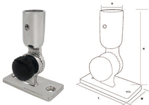
AISI316 STAINLESS STEEL ANTENNA BASE 316不锈钢天线座
