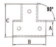
AISI316 STAINLESS STEEL 90°HANDRAIL TEE 316不锈钢90°直三通
