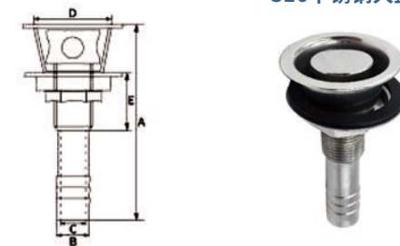
AISI316 STAINLESS STEEL TANK VENT WITH CAP 316不锈钢大盖出水口
